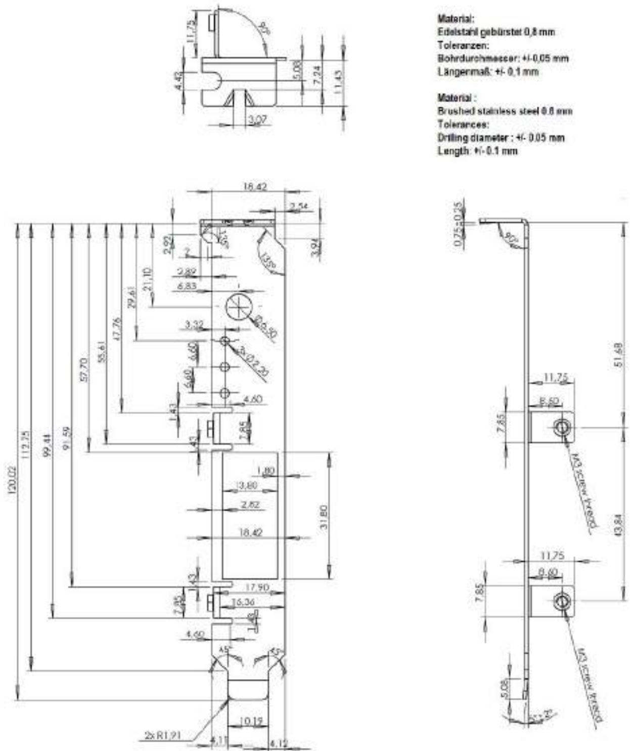
Figure 69: Dimensions Front Panel CIFX 50-RE, CIFX 50E-RE or CIFX 50E-RE/ET
