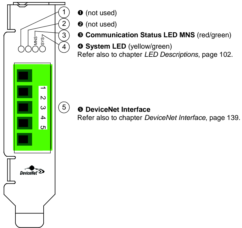
Figure 55: Front Plate CIFX 70E-DN, CIFX 70E-DNMR
